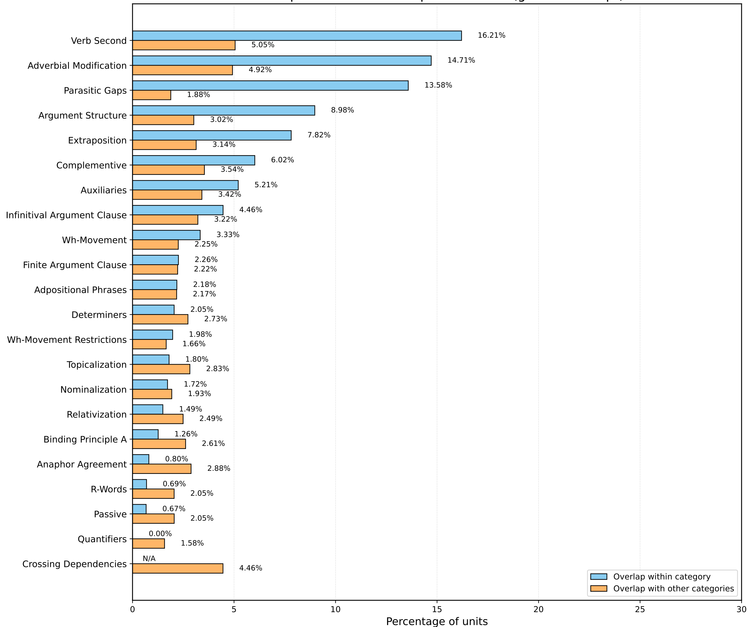
Cross-phenomenon overlap in BLiMP-NL (gemma-3-4b-pt)
